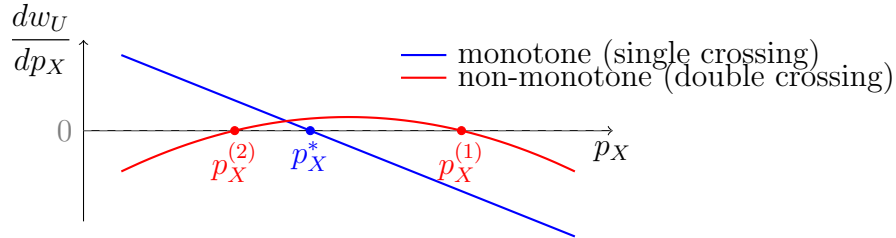
Figure 1: Local incidence of AI input prices on the unskilled wage: \frac{dw_U}{dp_X} vs. p_X . Above the zero line, unskilled wages rise with p_X ; below, they fall. A monotone path yields a single crossing (blue), while a non-monotone path yields two (red).
